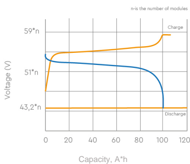
Charge/discharge at 25 °C, 0.5C
