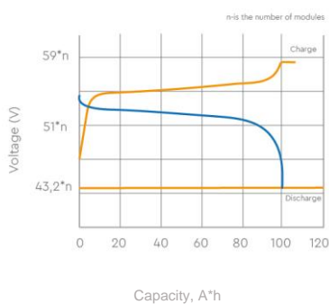
Charge/discharge at 25 °C, 0.5C
